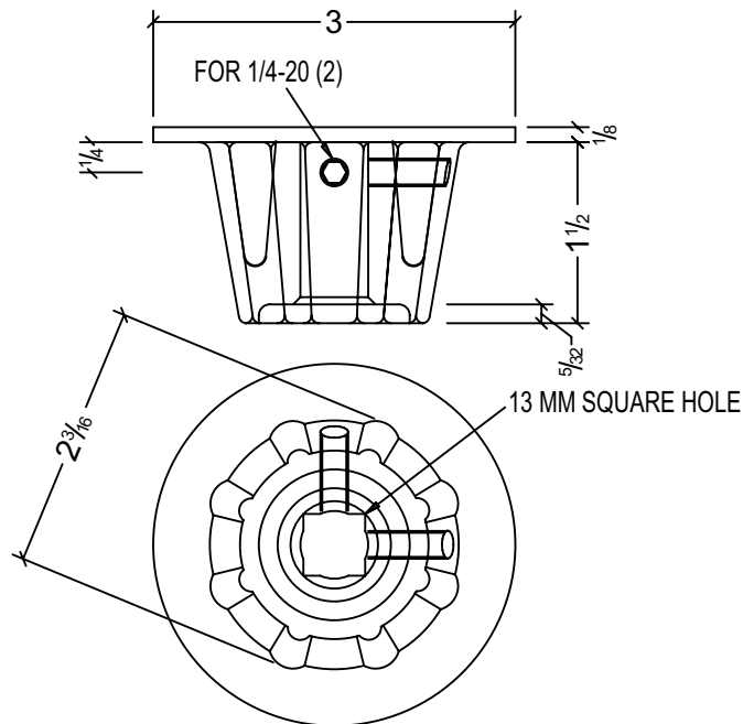
#278K NON REMOVABLE CONE (INV #415054)
