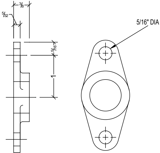
#278P BRONZE OILITE BUSHING (INV #407100)
