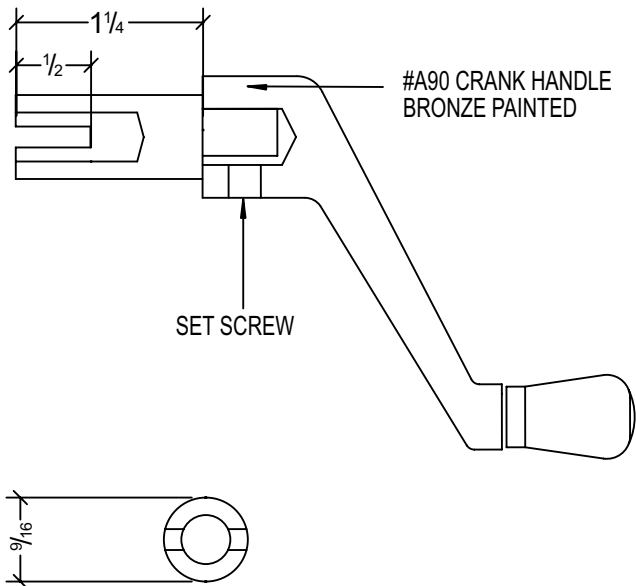
#278M REMOVABLE CRANK WITHOUT CONE OPERATION (INV #416502)
