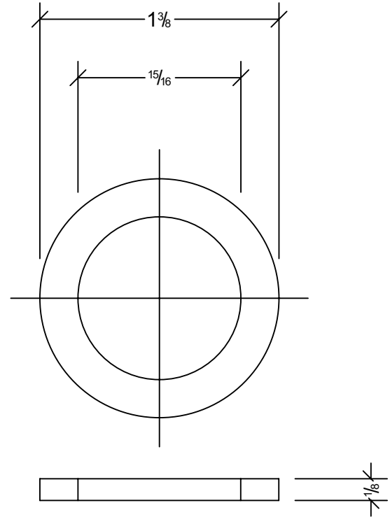
#278B WASHER (INV #494800) MATERIAL: CADMIUM PLATED STEEL
